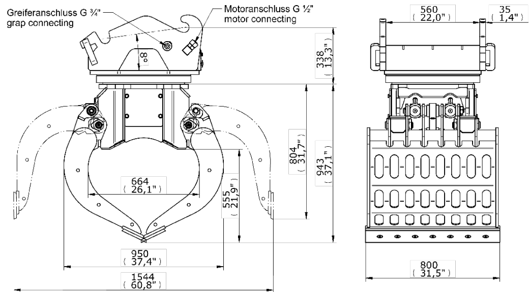
Screw-on Type
