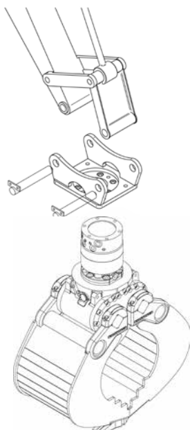
Grab with adapter for rigid mounting
